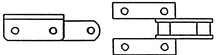
K-Style Chain
